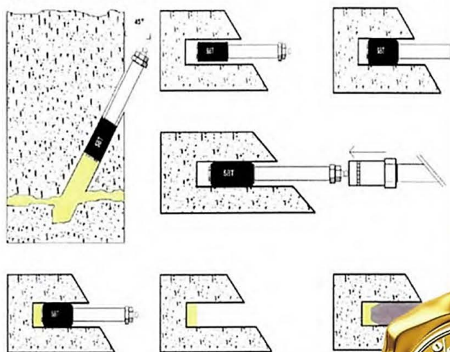
Typical Crack Injection Method
